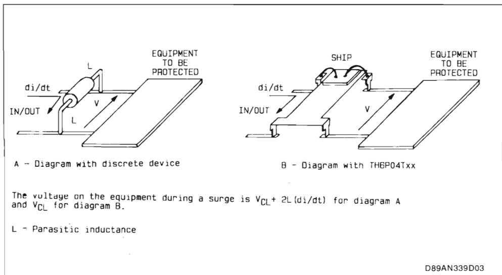
Figure 3 : Comparison between Discrete Device and TH6P04xx.
