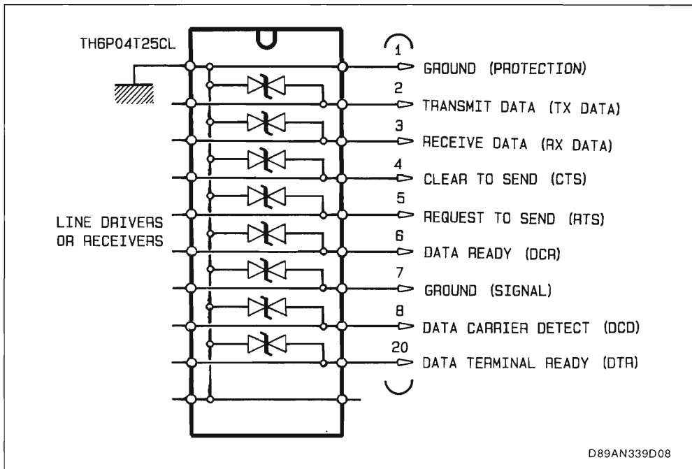
Figure 8 : RS232C Junction Protection.
