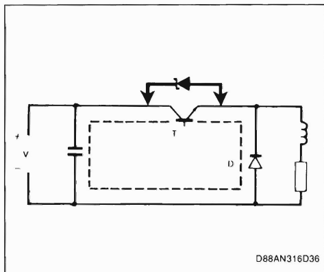
Figure 17 : The Transil Clamps the over Voltages l di/dt due to the unwanted Inductances l of the dotted Circuit.
