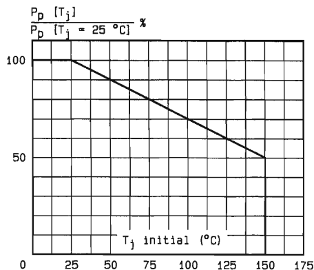
Fig.3 - Allowable power dissipation versus junction temperature.
