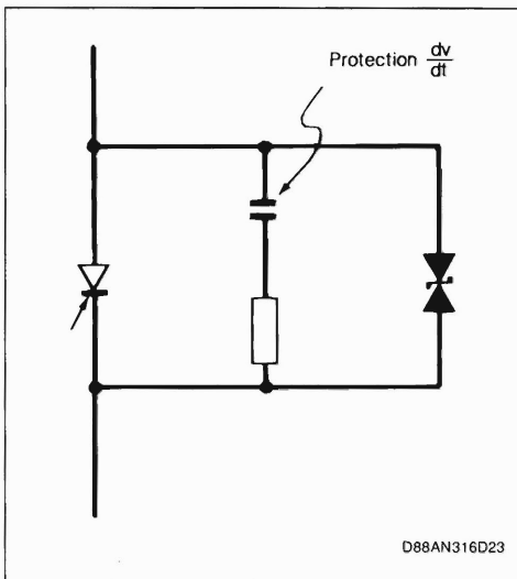
Figure 7 : Protection of Triacs.
