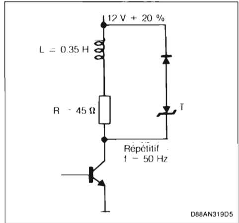
Figure 5 : Diagram of the Example with Real Values.
