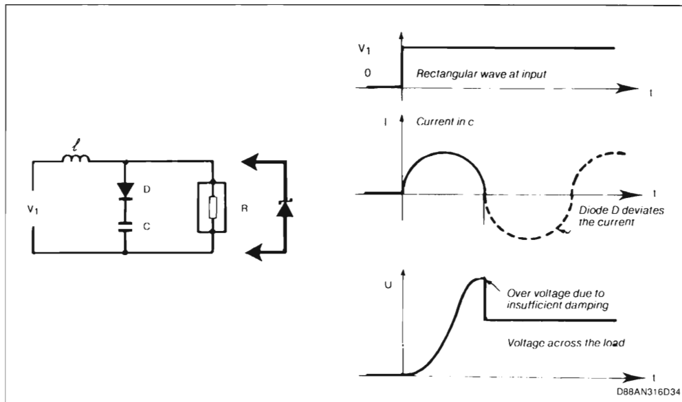
Figure 15 : Equivalent Diagram of the Clamping Circuit and Waveforms.
