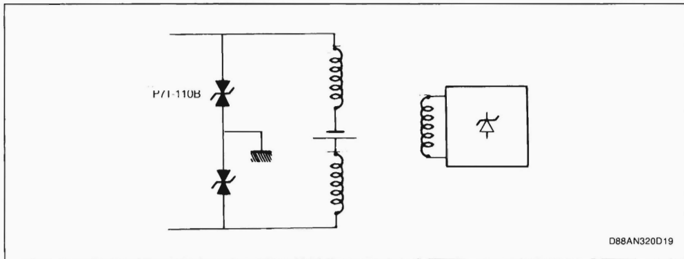
Figure 17 : PABX Protection.
