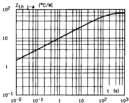
Fig.6 - Transient thermal impedance junction-ambient for mounting n°2 versus pulse duration ( L = 10 \text{ mm} ).
