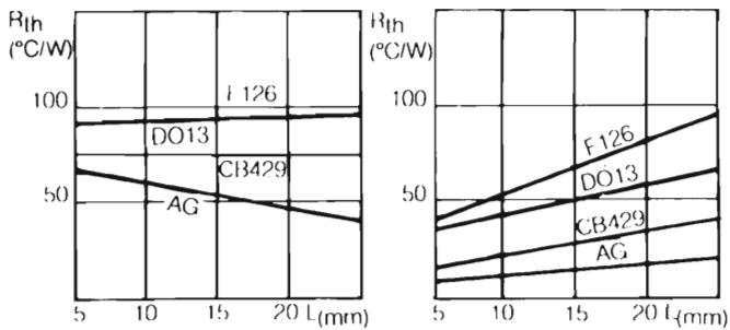
Figure 6 : Thermal Resistance Junction-ambient According to Connections Length. Left : Assembly on Printed Circuit. Right : Assembly on Infinite Heatsink.
