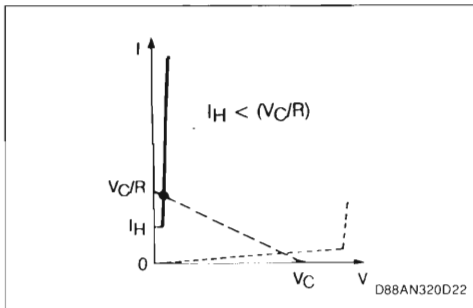
Figure 19 : Wrong Choice of the Trisil for DC Operation.
