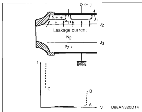
Figure 12 : Operation in the Blocked Mode.
