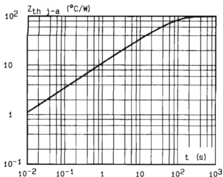
Fig.6 - Transient thermal impedance junction-ambient versus pulse duration.
