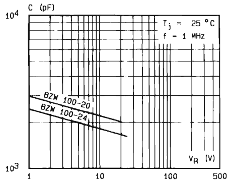
Fig.8 - Capacitance versus reverse applied voltage (typical values).
