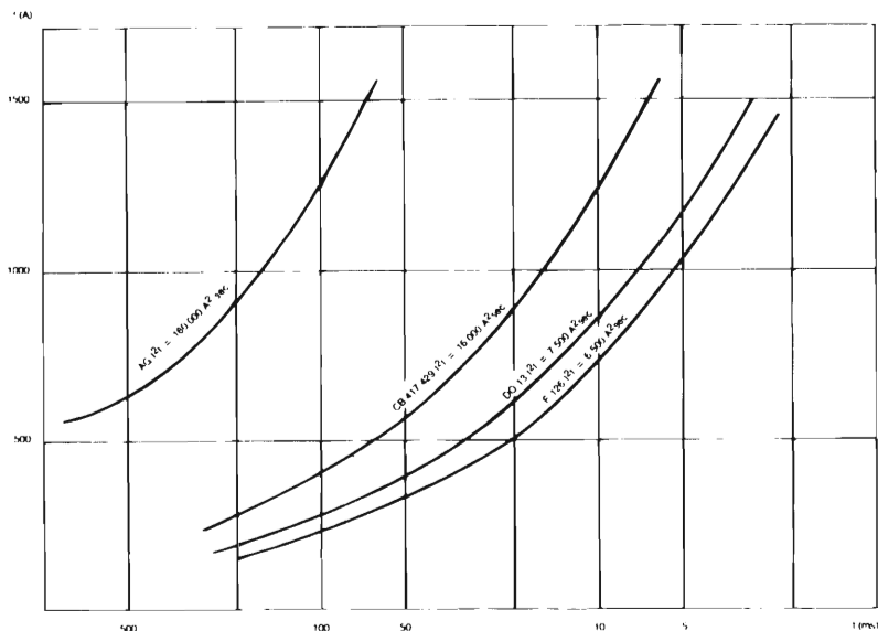
Figure 1 : Limit of the current which does not result in an open circuit for a TRANSIL diode. By analogy with fuses, these limits can be characterized within the 10 \mu s to 1 s interval by I^2t ( A^2 \cdot sec ).
