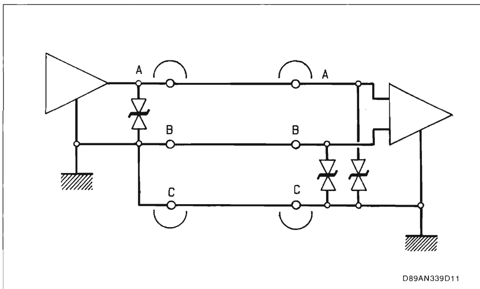
Figure 11 : RS423 Principle of Protection.
