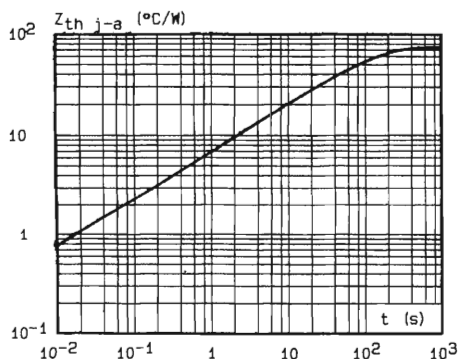
Fig.6 - Transient thermal impedance junction-ambient for mounting n°2 versus pulse duration ( L = 10 mm).
