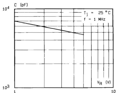
Fig.8 - Capacitance versus reverse applied voltage (typical values).
