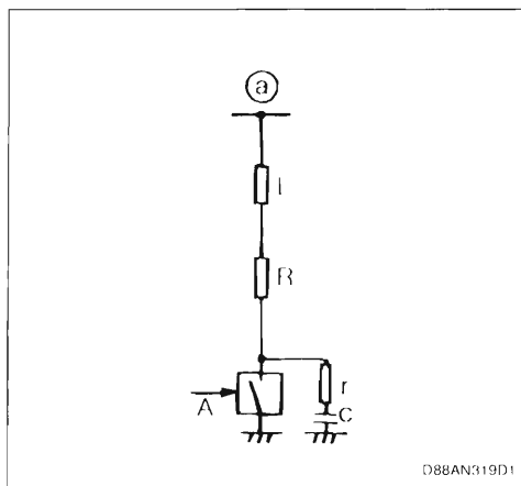
Figure 1 : Relay Drive Protection by R.C. Network.
