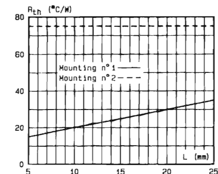
Fig.5 - Thermal resistance versus lead length.
