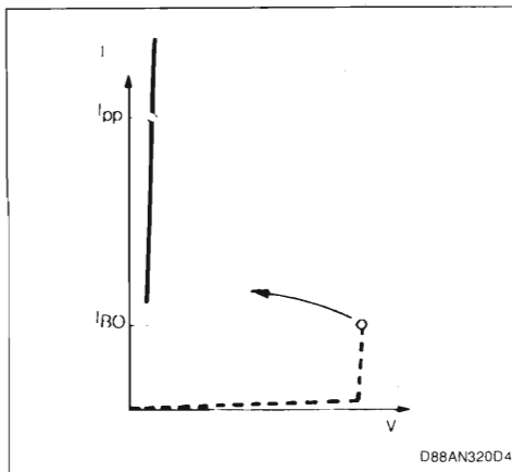
Figure 4 : Triggering Characteristics.
