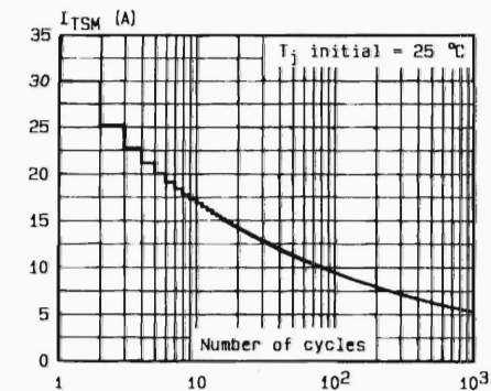
Fig.4 - Non repetitive surge peak on-state current versus number of cycles.
