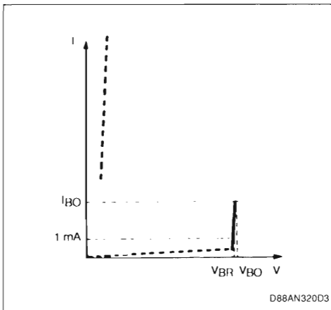
Figure 3 : Avalanche Characteristic of the Trisil.
