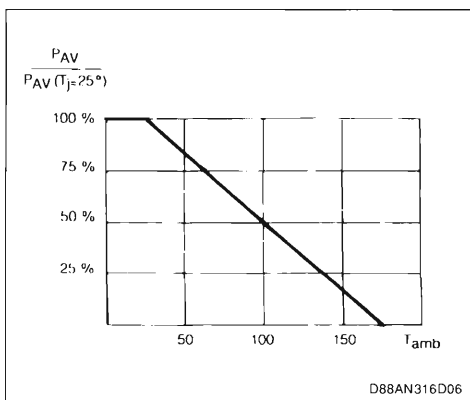
Figure 6 : Maximum Average Power as a Function of Ambient Temperature.
