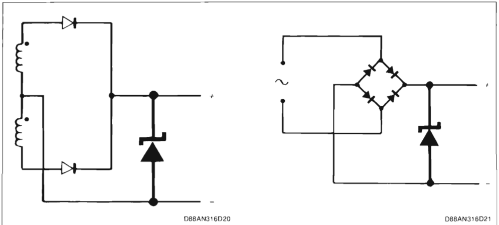
Figure 3 : Optimal Solution. A single Transil protects the rectifying components whatever the origin (power supply or load) of the over voltages.
