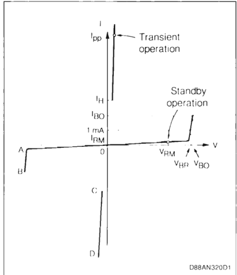
Figure 2 : Low Level Characteristics.
