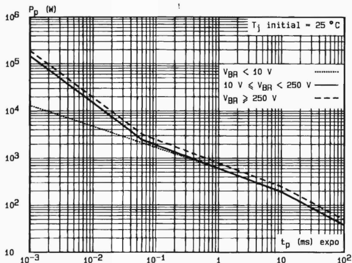
Fig. 1 - Peak power versus exponential pulse duration.
