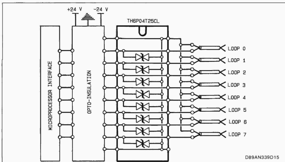
Figure 15 : 8 Ways Driver or Receiver Loops.
