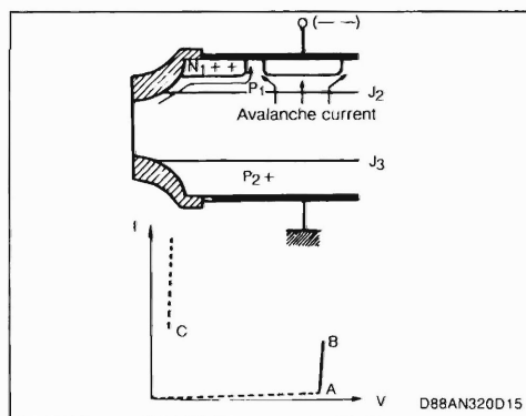
Figure 13 : Operation in the Avalanche Mode.
