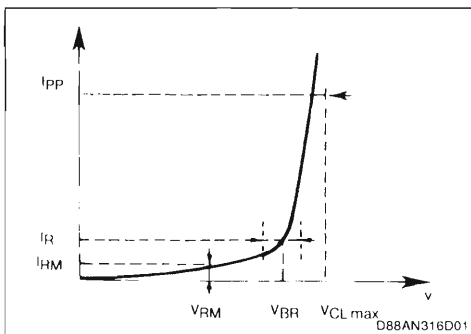
Figure 1 : Main Characteristics of a Transil.
