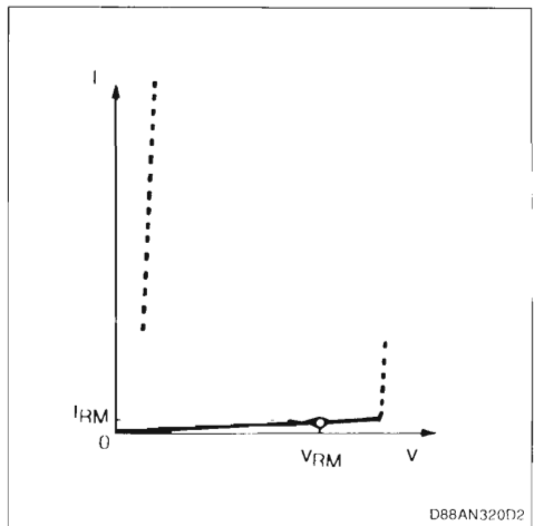
Figure 2 : Low Level Characteristics.
