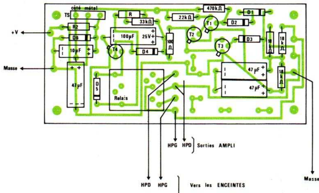
Figure 4. – Implantation des composants.
