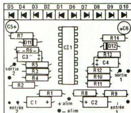
Figure 13. - Implantation des composants.
